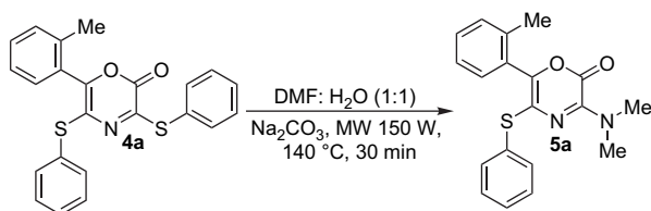
Scheme 2. Dimethylation of oxazinone 4a .
