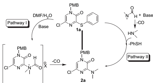
Scheme 3. Plausible mechanisms for the amination protocol.
