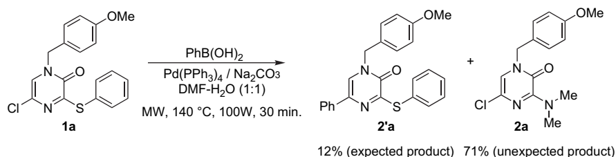
Scheme 1. Attempted arylation of 5-chloro substituted pyrazin-2(1H)-one ( 1a ).
